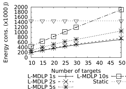
Figure 14: Total energy consumption for different detection frequencies.
